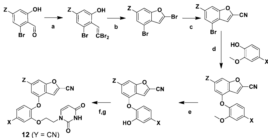
Scheme 3. Synthesis of the 2-Cyanobenzofurans
